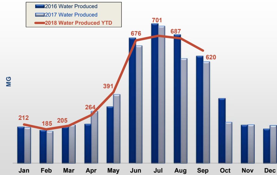
Water Treatment Plant Monthly Production
